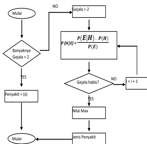
Gambar 2. Flowchart Perhitungan Teorema Bayes
